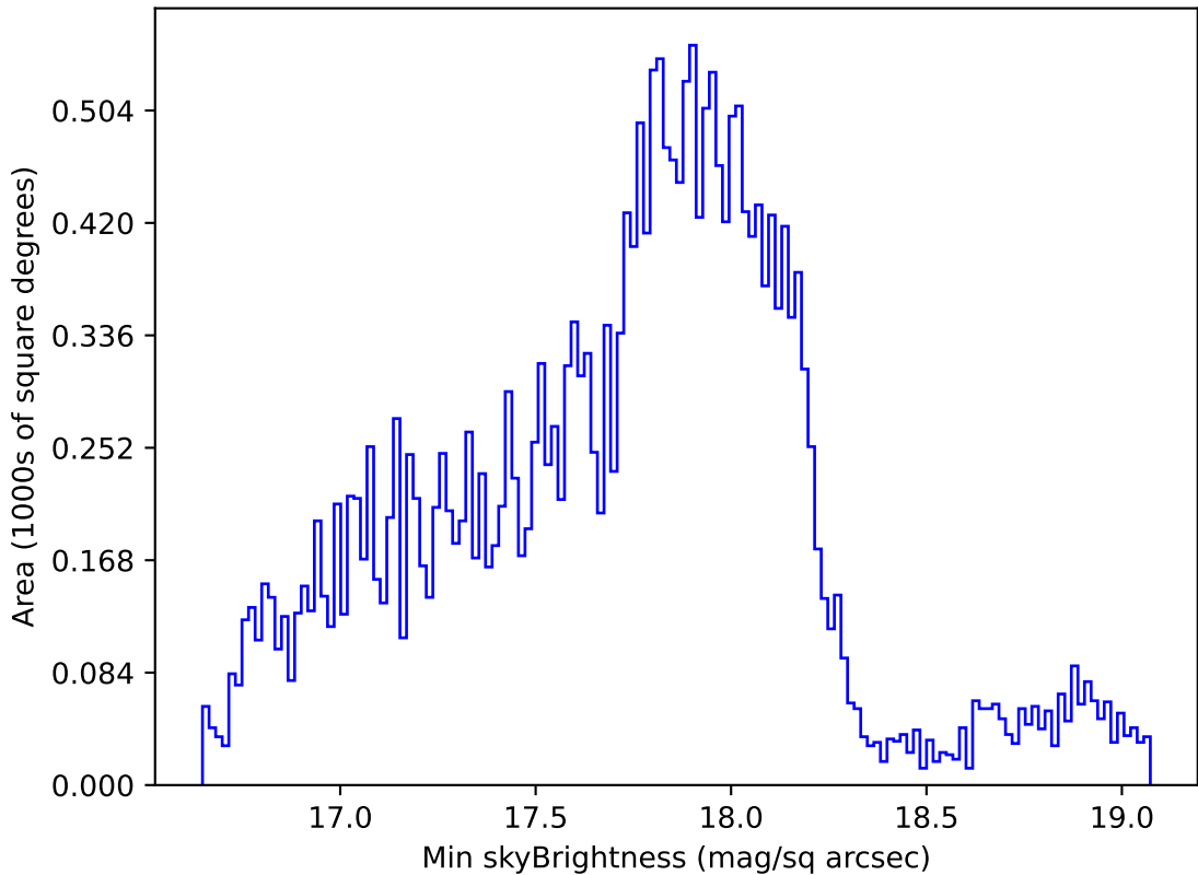
too_elab_r8_d3_ugrizy_v3.4_10yrs Yr 1 all bands: Min skyBrightness
