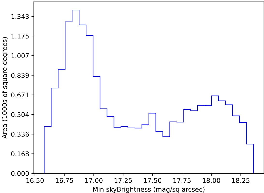
too_elab_r8_d3_ugrizy_v3.4_10yrs WFD z band: Min skyBrightness
