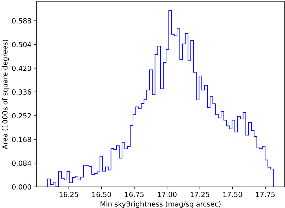
too_elab_r8_d3_ugrizy_v3.4_10yrs WFD y band: Min skyBrightness
