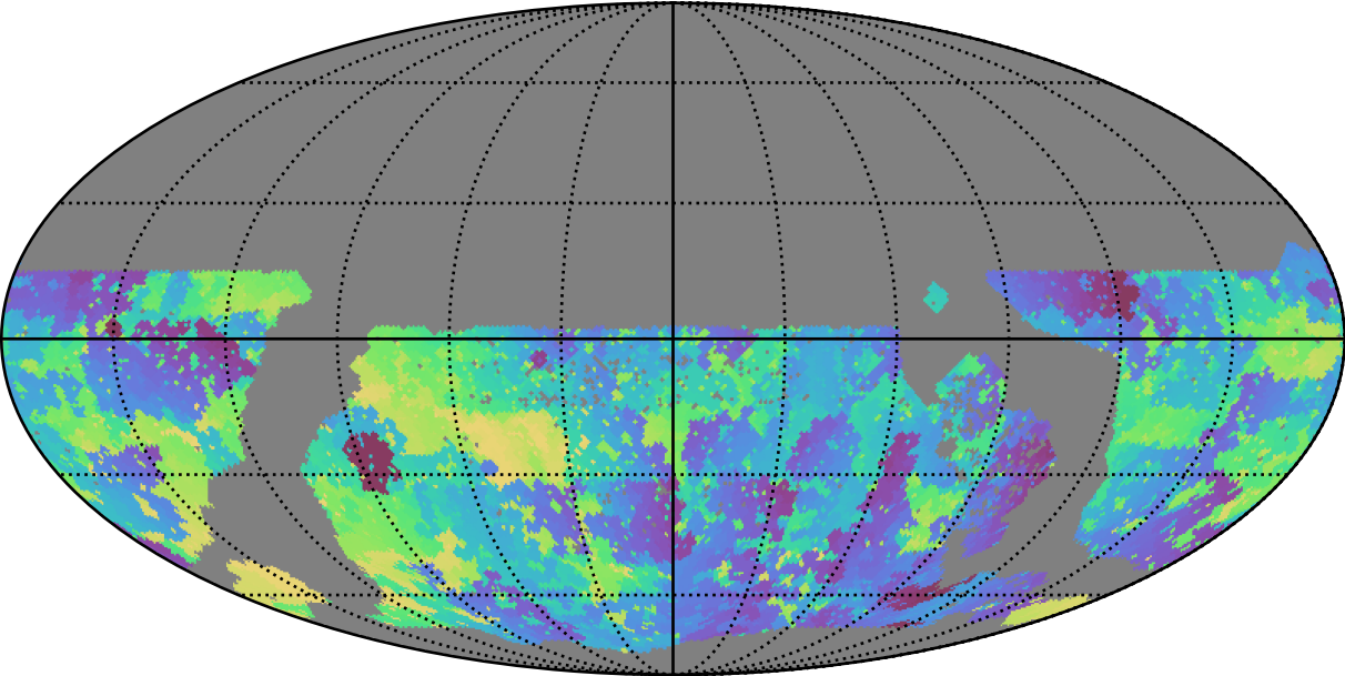
too_elab_r8_d3_ugrizy_v3.4_10yrs WFD u band: Min skyBrightness
