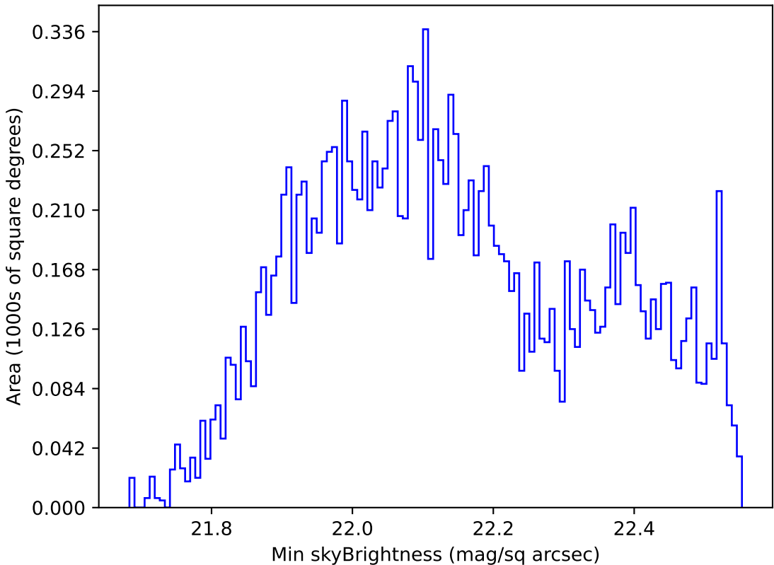
too_elab_r8_d3_ugrizy_v3.4_10yrs WFD u band: Min skyBrightness
