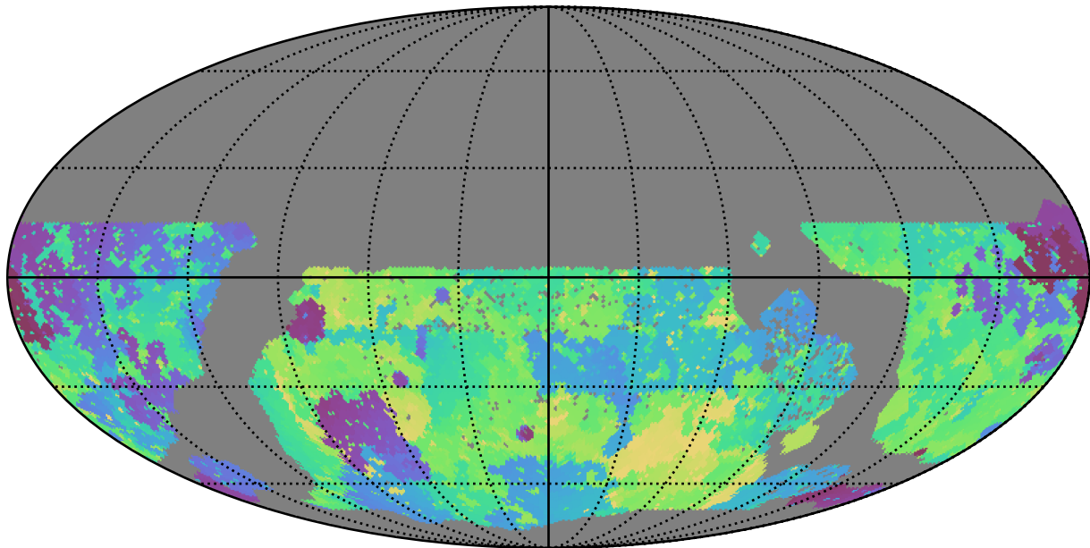
too_elab_r8_d3_ugrizy_v3.4_10yrs WFD g band: Min skyBrightness
