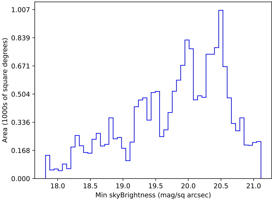
too_elab_r8_d3_ugrizy_v3.4_10yrs WFD g band: Min skyBrightness
