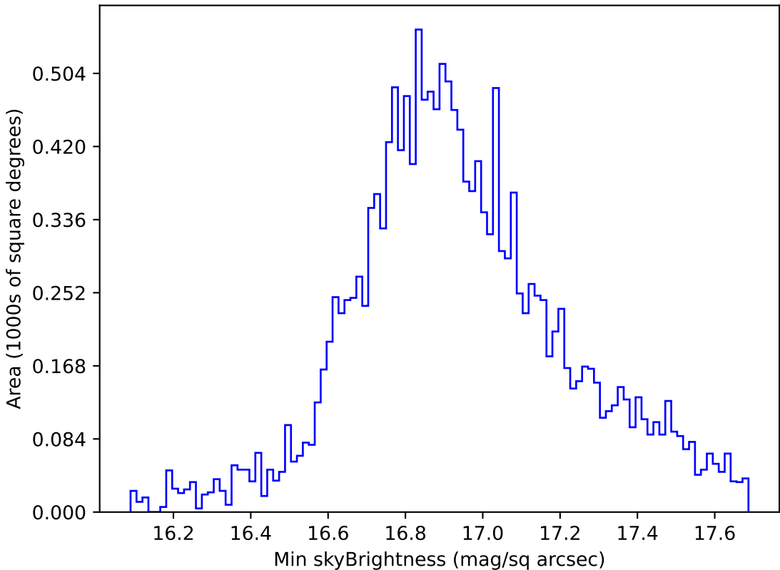
too_elab_r8_d3_ugrizy_v3.4_10yrs WFD all bands: Min skyBrightness
