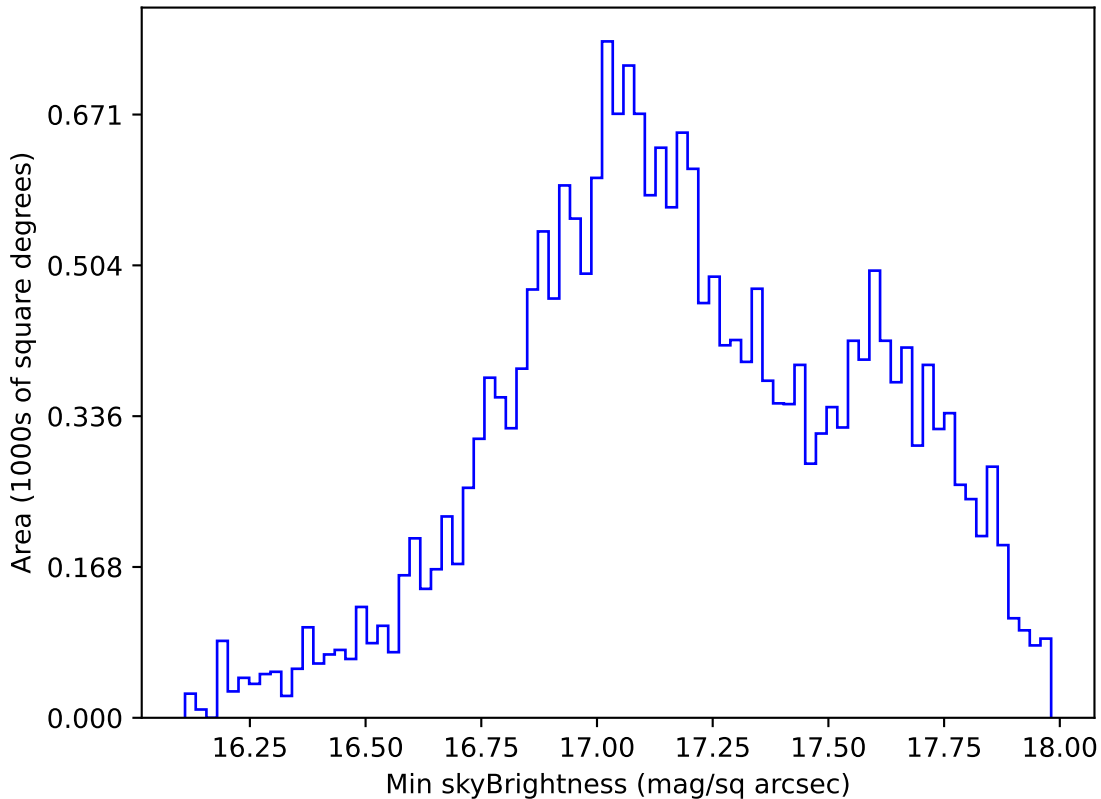
too_elab_r8_d3_ugrizy_v3.4_10yrs All sky y band: Min skyBrightness
