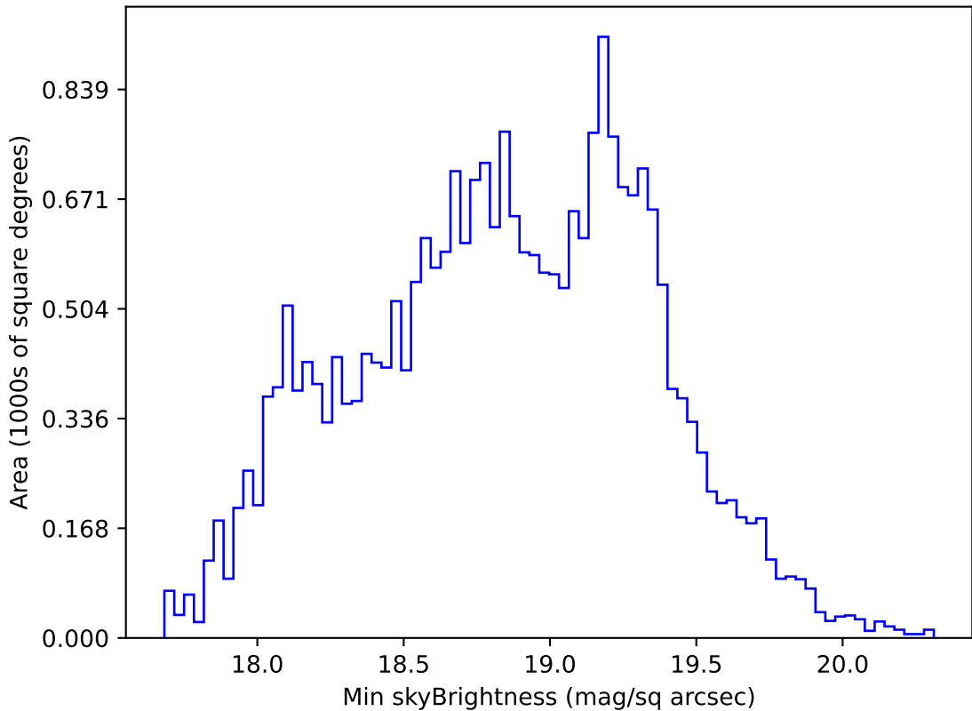
too_elab_r8_d3_ugrizy_v3.4_10yrs All sky r band: Min skyBrightness
