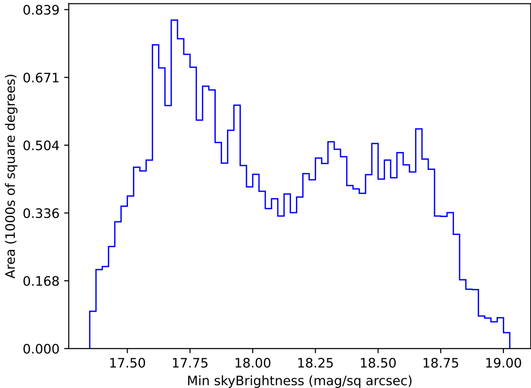
too_elab_r8_d3_ugrizy_v3.4_10yrs All sky i band: Min skyBrightness
