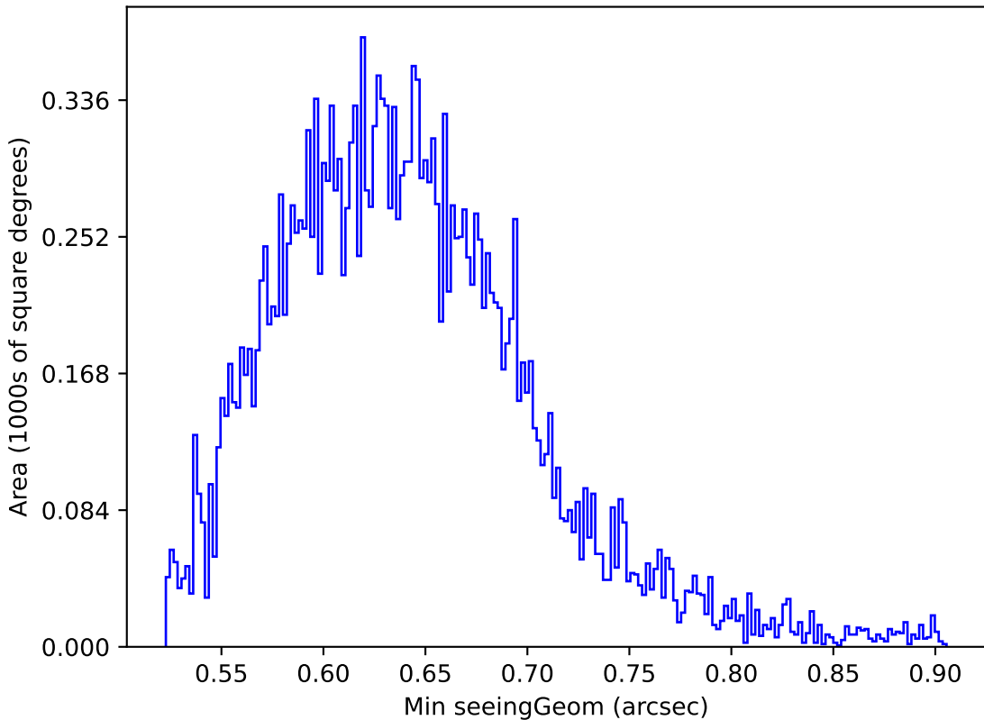
too_elab_r8_d3_ugrizy_v3.4_10yrs Yr 1 y band: Min seeingGeom
