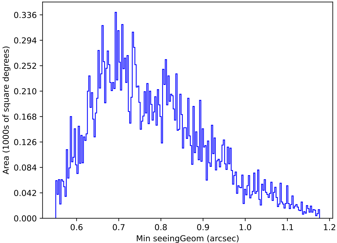
too_elab_r8_d3_ugrizy_v3.4_10yrs Yr 1 u band: Min seeingGeom
