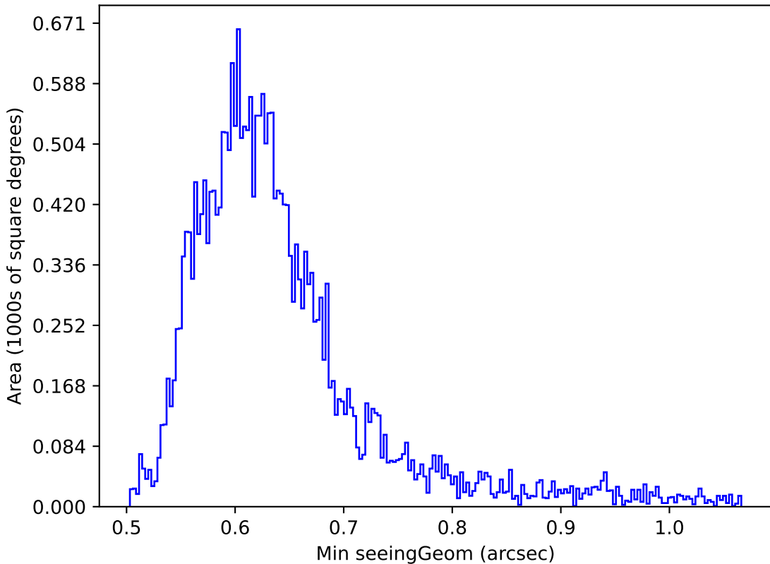
too_elab_r8_d3_ugrizy_v3.4_10yrs Yr 1 r band: Min seeingGeom
