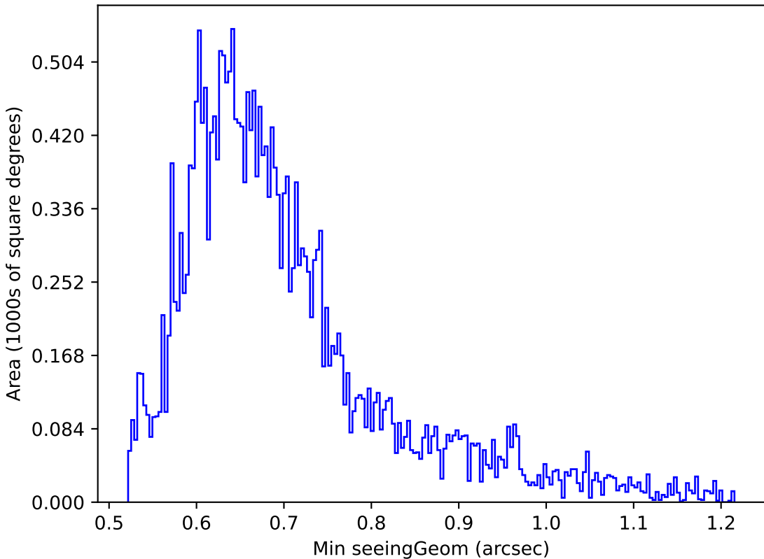
too_elab_r8_d3_ugrizy_v3.4_10yrs Yr 1 g band: Min seeingGeom
