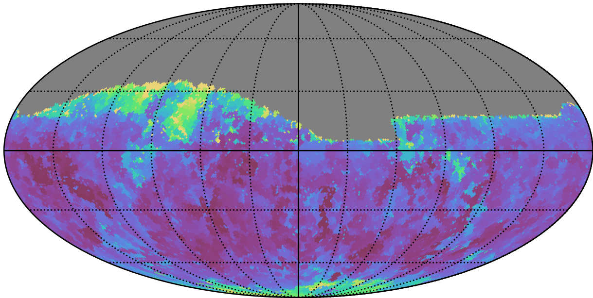
too_elab_r8_d3_ugrizy_v3.4_10yrs Yr 1 z band: Min seeingEff
