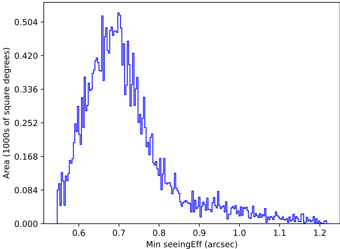
too_elab_r8_d3_ugrizy_v3.4_10yrs Yr 1 z band: Min seeingEff
