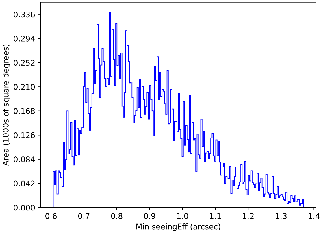
too_elab_r8_d3_ugrizy_v3.4_10yrs Yr 1 u band: Min seeingEff
