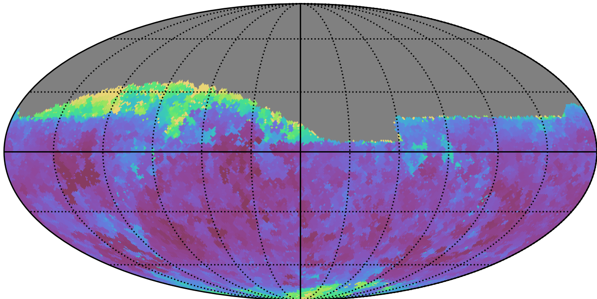
too_elab_r8_d3_ugrizy_v3.4_10yrs Yr 1 i band: Min seeingEff
