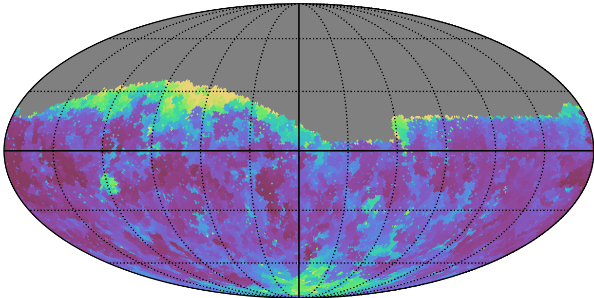
too_elab_r8_d3_ugrizy_v3.4_10yrs Yr 1 g band: Min seeingEff
