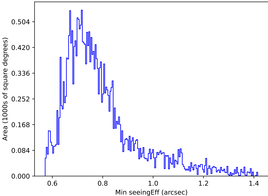
too_elab_r8_d3_ugrizy_v3.4_10yrs Yr 1 g band: Min seeingEff
