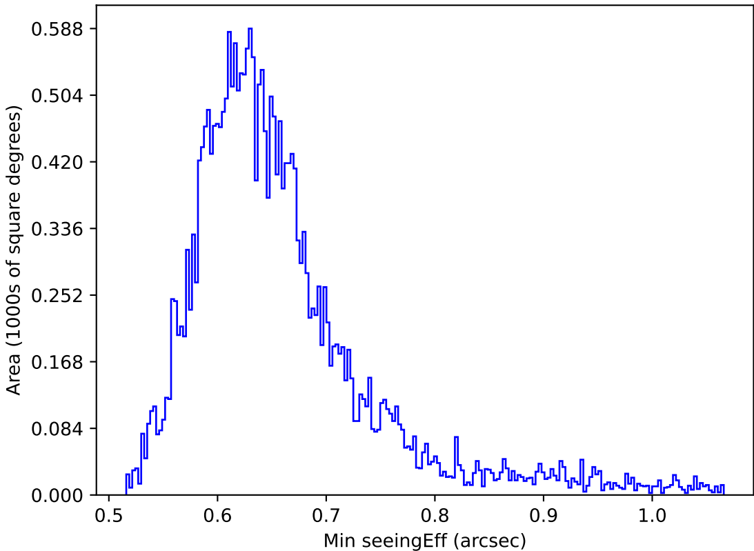
too_elab_r8_d3_ugrizy_v3.4_10yrs Yr 1 all bands: Min seeingEff
