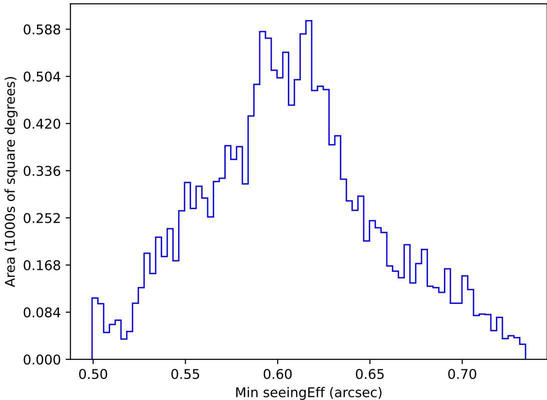
too_elab_r8_d3_ugrizy_v3.4_10yrs WFD z band: Min seeingEff
