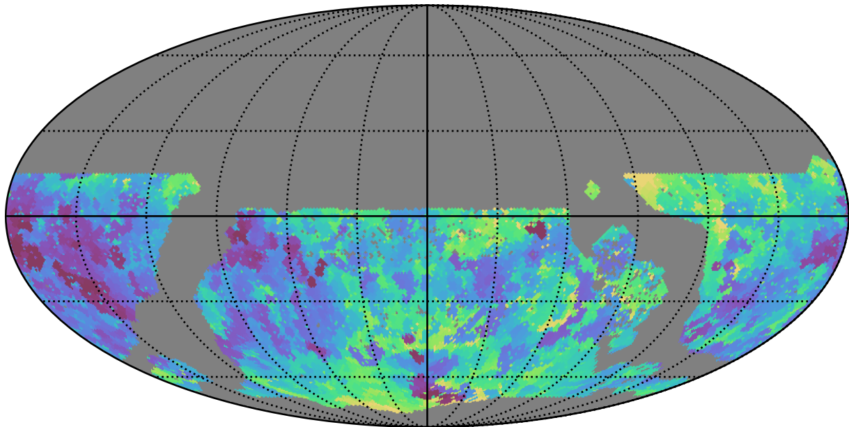
too_elab_r8_d3_ugrizy_v3.4_10yrs WFD u band: Min seeingEff
