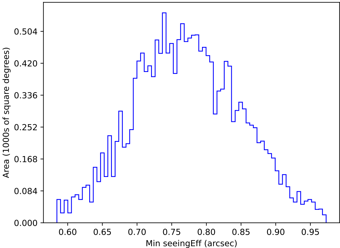
too_elab_r8_d3_ugrizy_v3.4_10yrs WFD u band: Min seeingEff
