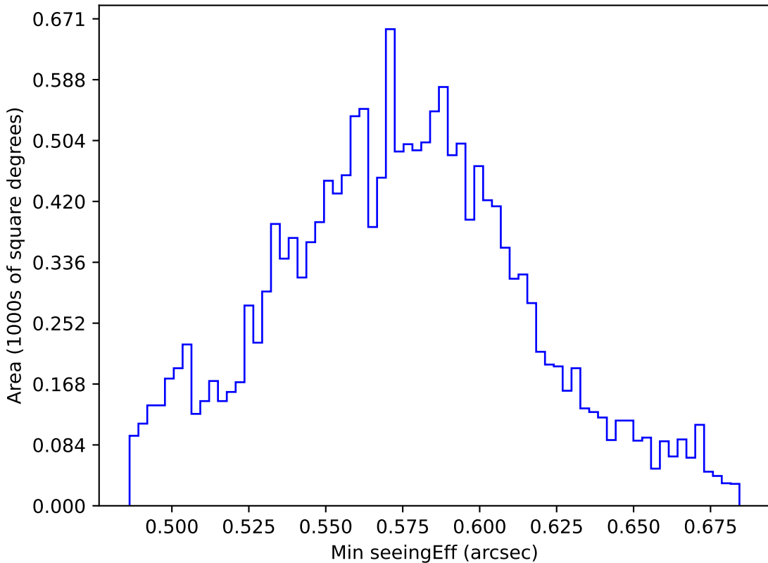
too_elab_r8_d3_ugrizy_v3.4_10yrs WFD all bands: Min seeingEff
