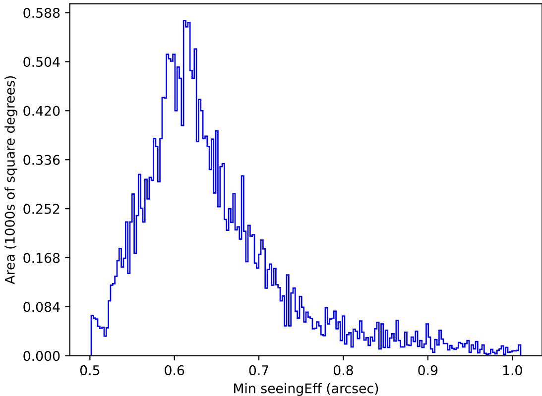
too_elab_r8_d3_ugrizy_v3.4_10yrs All sky z band: Min seeingEff
