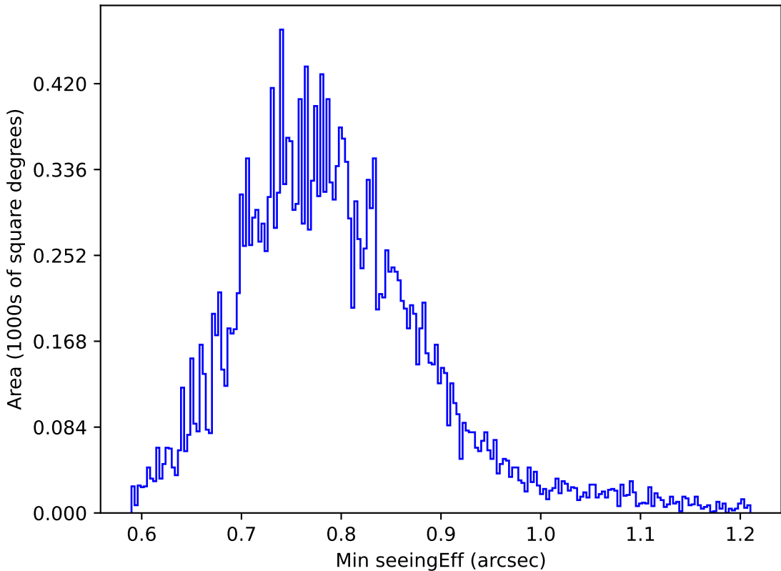
too_elab_r8_d3_ugrizy_v3.4_10yrs All sky u band: Min seeingEff
