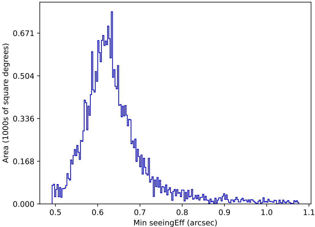
too_elab_r8_d3_ugrizy_v3.4_10yrs All sky r band: Min seeingEff
