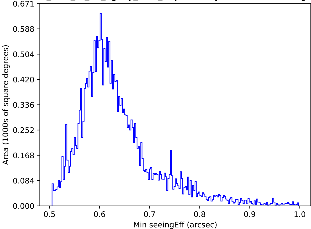
too_elab_r8_d3_ugrizy_v3.4_10yrs All sky i band: Min seeingEff
