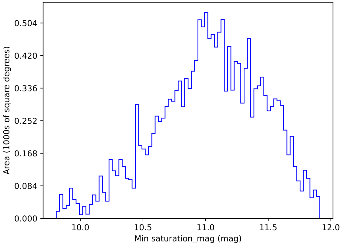
too_elab_r8_d3_ugrizy_v3.4_10yrs WFD all bands: Min saturation_mag
