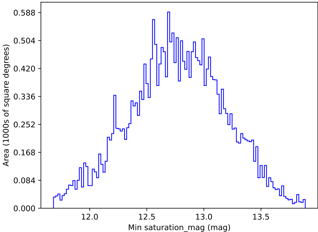
too_elab_r8_d3_ugrizy_v3.4_10yrs All sky g band: Min saturation_mag
