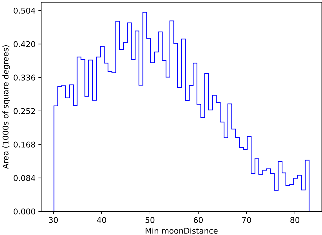
too_elab_r8_d3_ugrizy_v3.4_10yrs WFD u band: Min moonDistance
