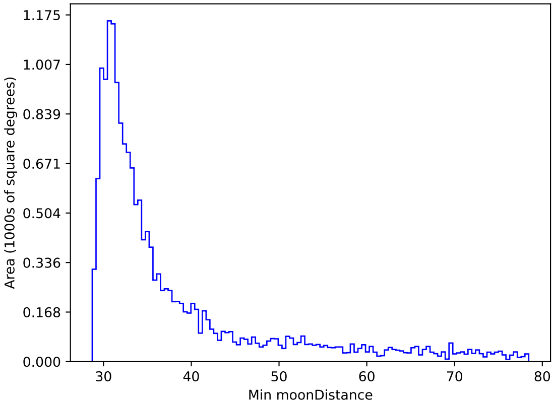
too_elab_r8_d3_ugrizy_v3.4_10yrs WFD r band: Min moonDistance
