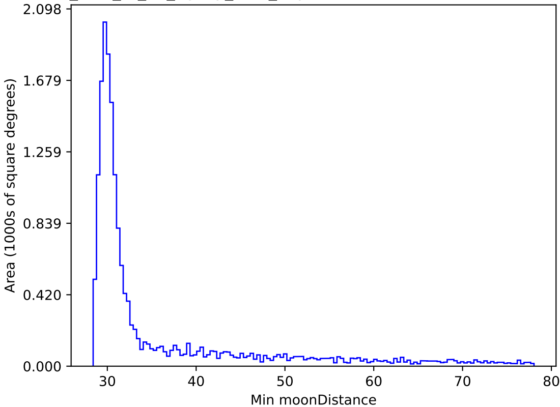
too_elab_r8_d3_ugrizy_v3.4_10yrs WFD i band: Min moonDistance
