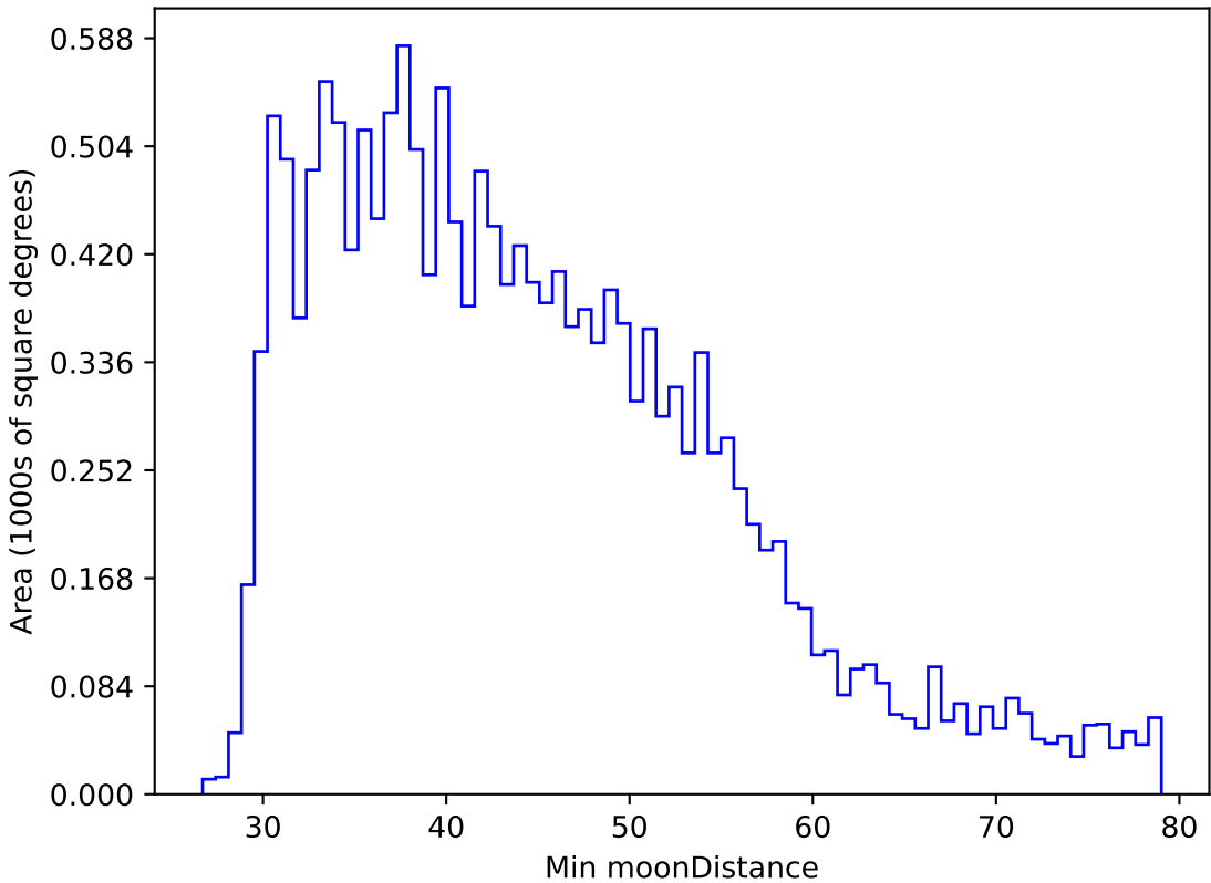
too_elab_r8_d3_ugrizy_v3.4_10yrs WFD g band: Min moonDistance
