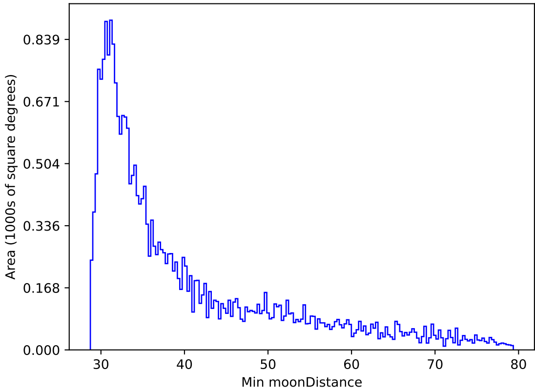
too_elab_r8_d3_ugrizy_v3.4_10yrs All sky r band: Min moonDistance
