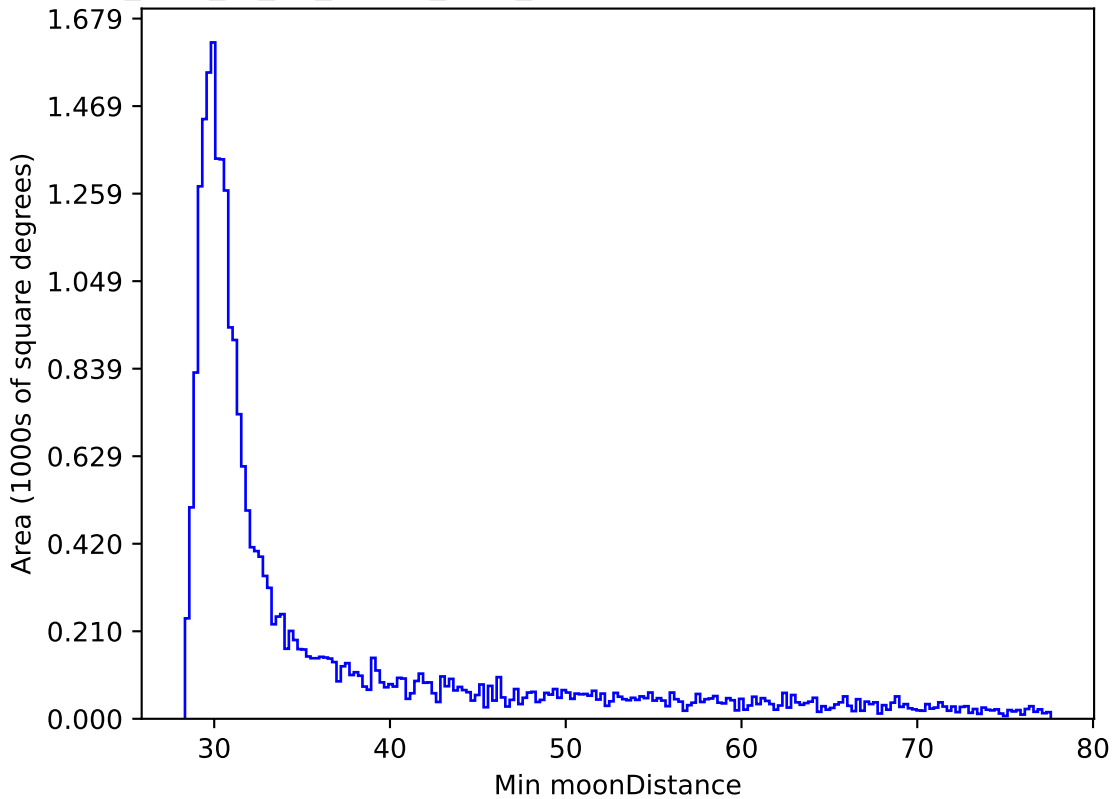
too_elab_r8_d3_ugrizy_v3.4_10yrs All sky i band: Min moonDistance
