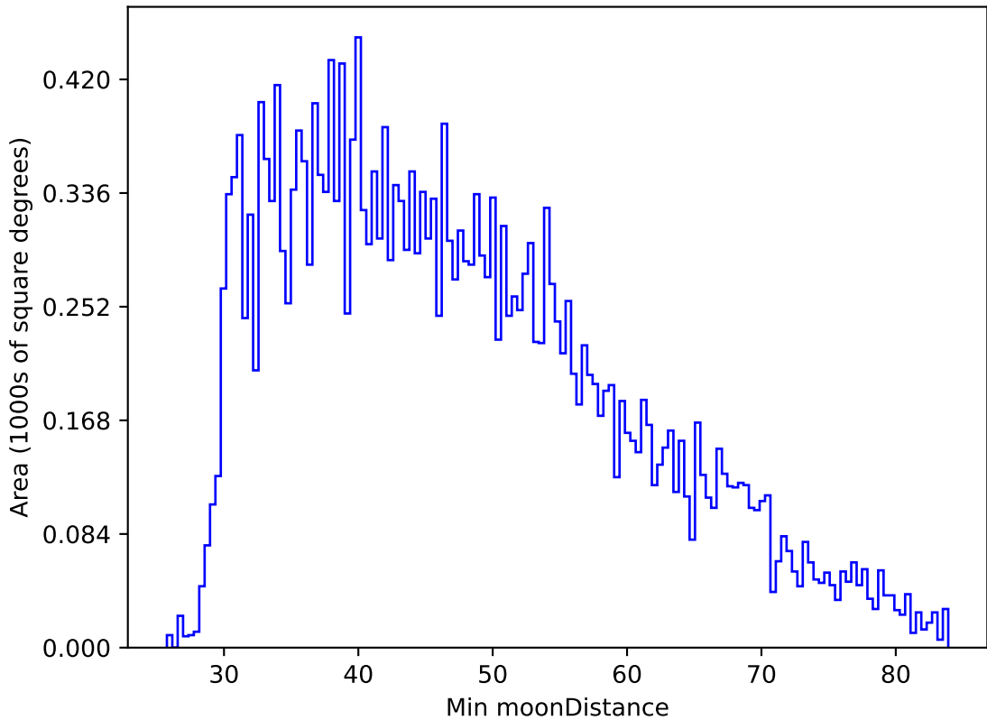
too_elab_r8_d3_ugrizy_v3.4_10yrs All sky g band: Min moonDistance
