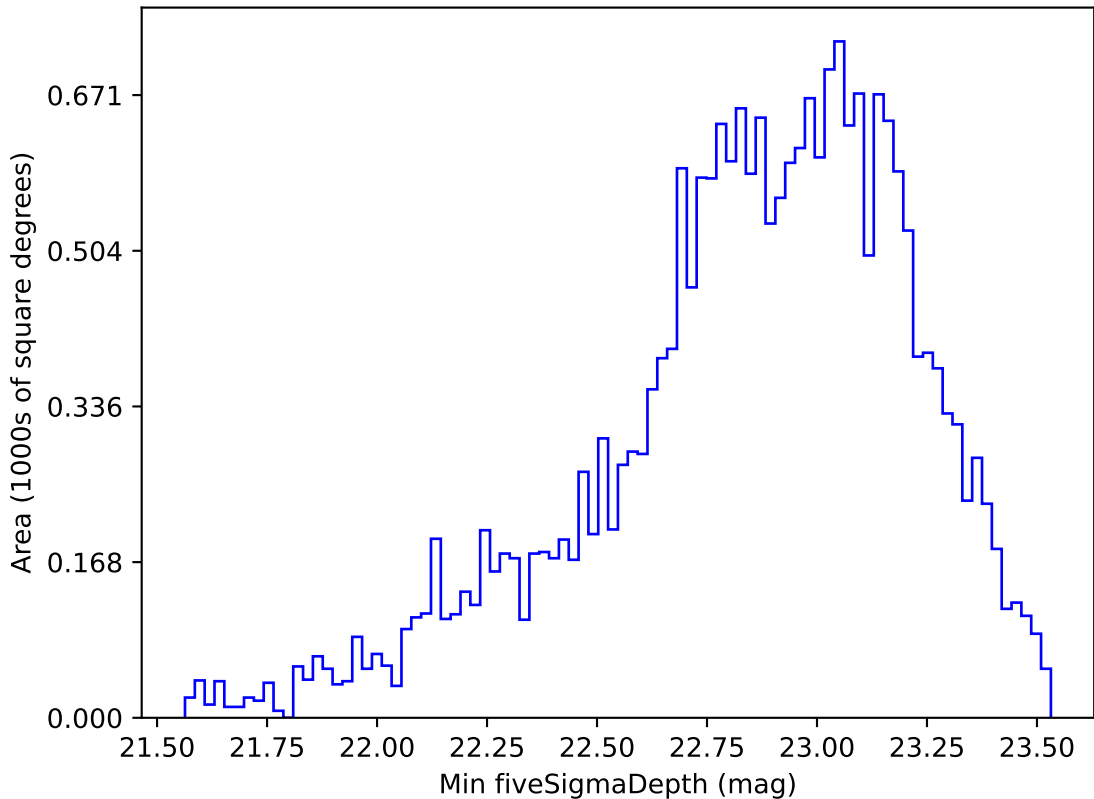
too_elab_r8_d3_ugrizy_v3.4_10yrs Yr 1 u band: Min fiveSigmaDepth
