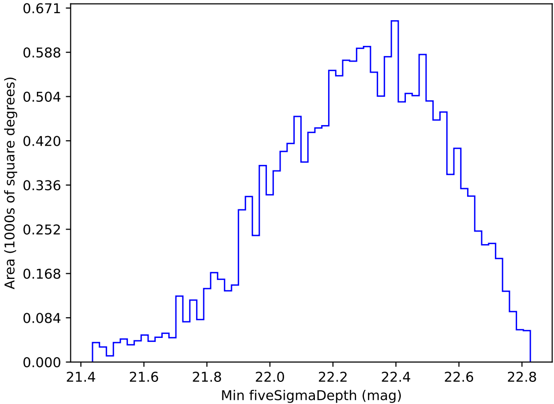
too_elab_r8_d3_ugrizy_v3.4_10yrs WFD u band: Min fiveSigmaDepth
