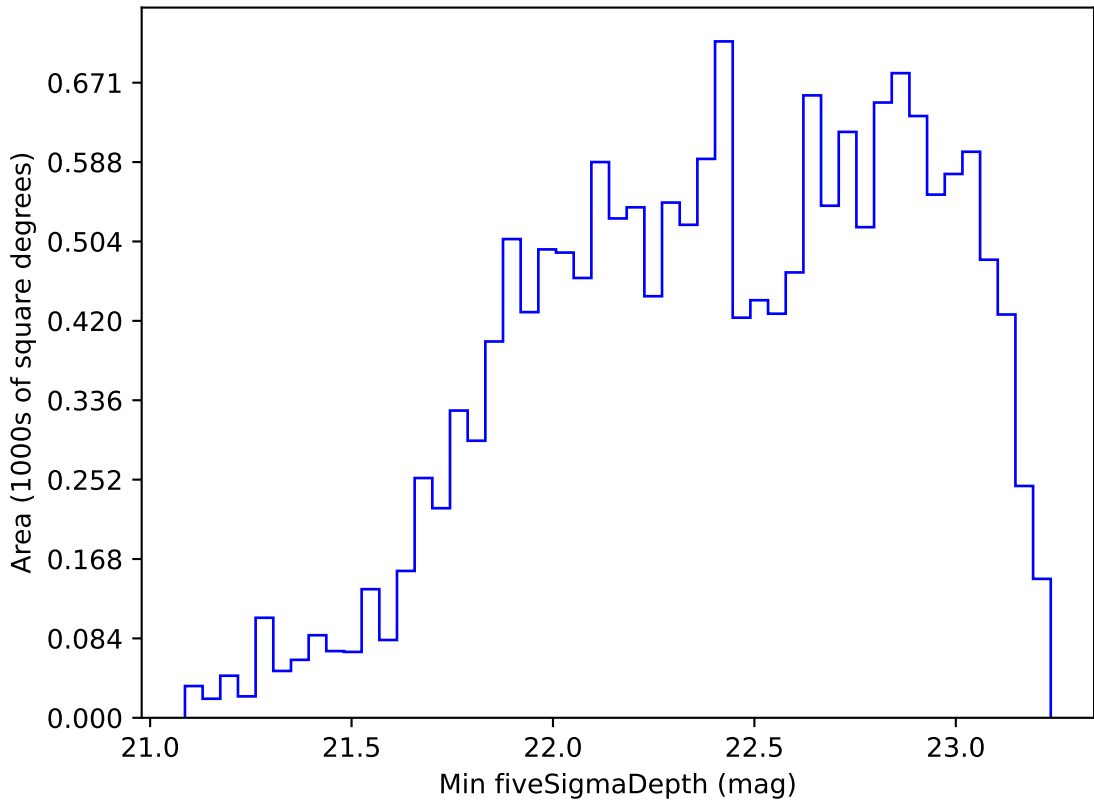
too_elab_r8_d3_ugrizy_v3.4_10yrs WFD r band: Min fiveSigmaDepth
