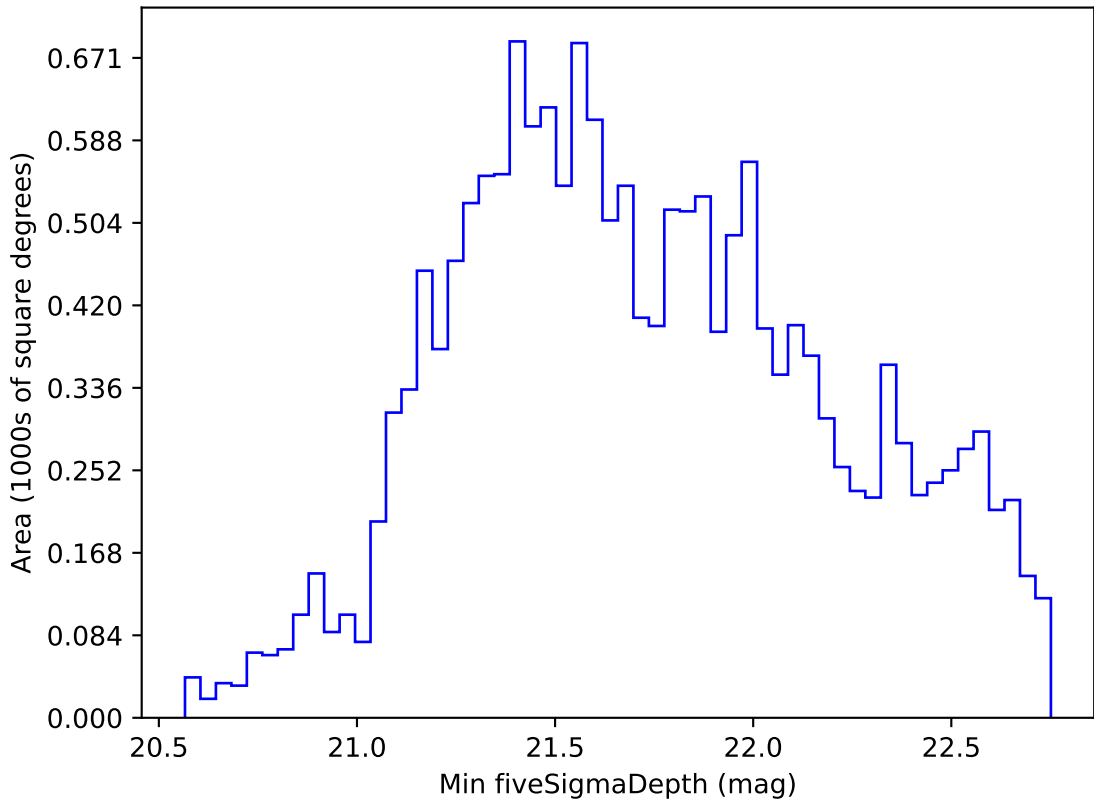
too_elab_r8_d3_ugrizy_v3.4_10yrs WFD i band: Min fiveSigmaDepth
