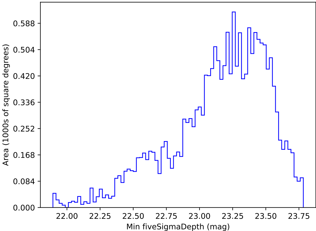
too_elab_r8_d3_ugrizy_v3.4_10yrs WFD g band: Min fiveSigmaDepth
