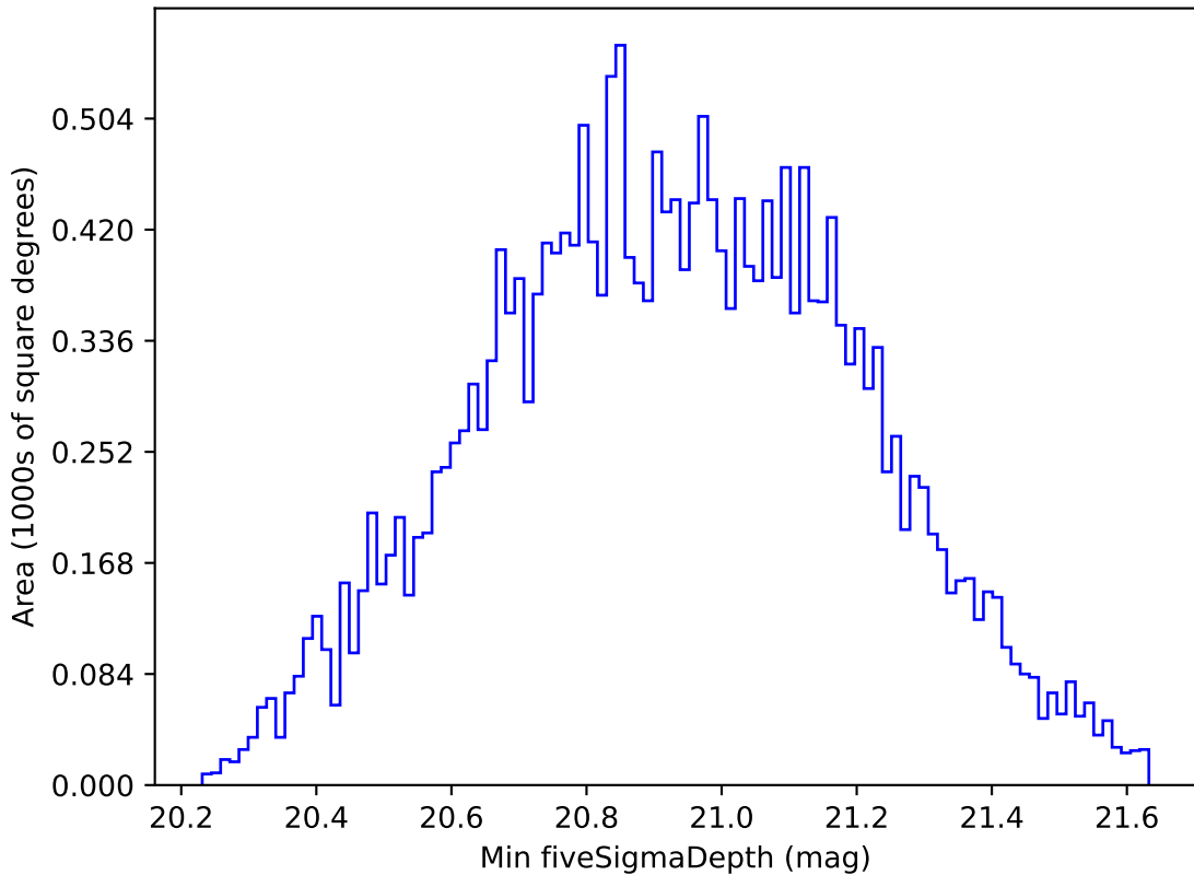
too_elab_r8_d3_ugrizy_v3.4_10yrs All sky y band: Min fiveSigmaDepth
