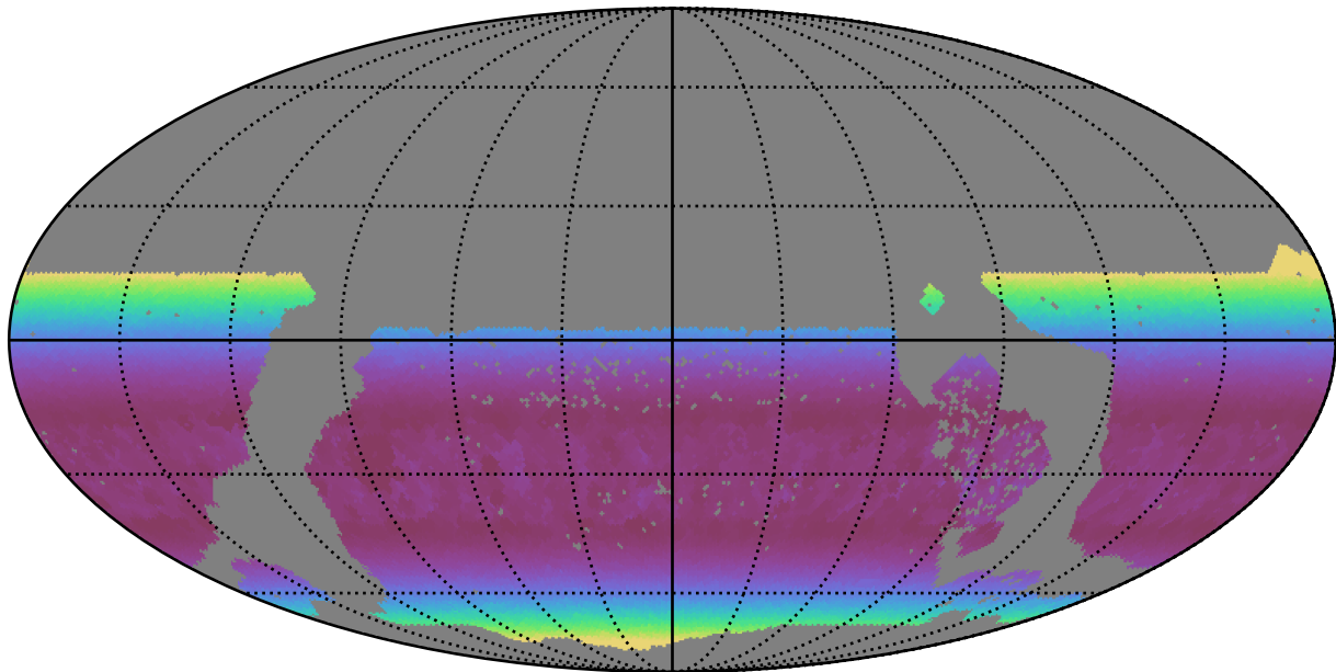
too_elab_r8_d3_ugrizy_v3.4_10yrs WFD u band: Min airmass
