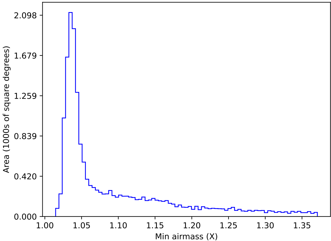
too_elab_r8_d3_ugrizy_v3.4_10yrs WFD g band: Min airmass
