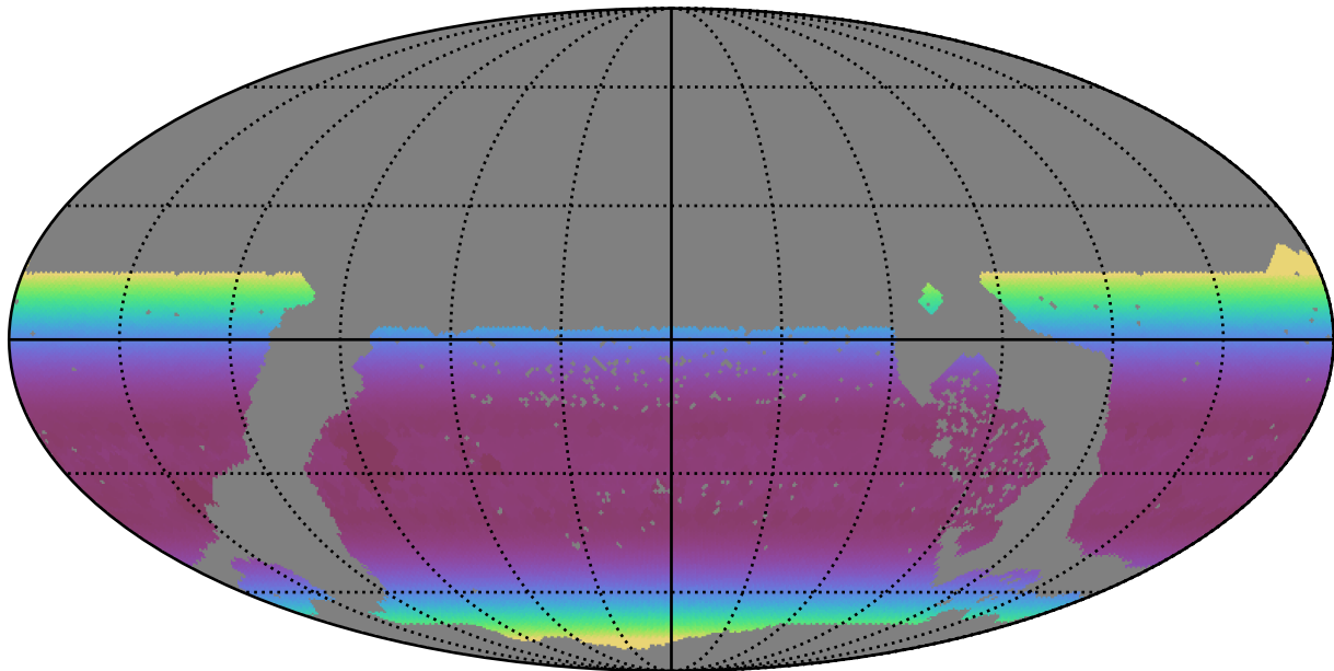
too_elab_r8_d3_ugrizy_v3.4_10yrs WFD all bands: Min airmass
