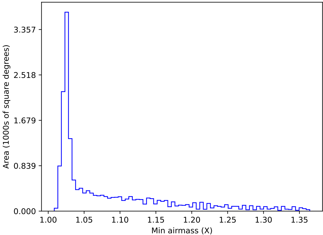
too_elab_r8_d3_ugrizy_v3.4_10yrs WFD all bands: Min airmass
