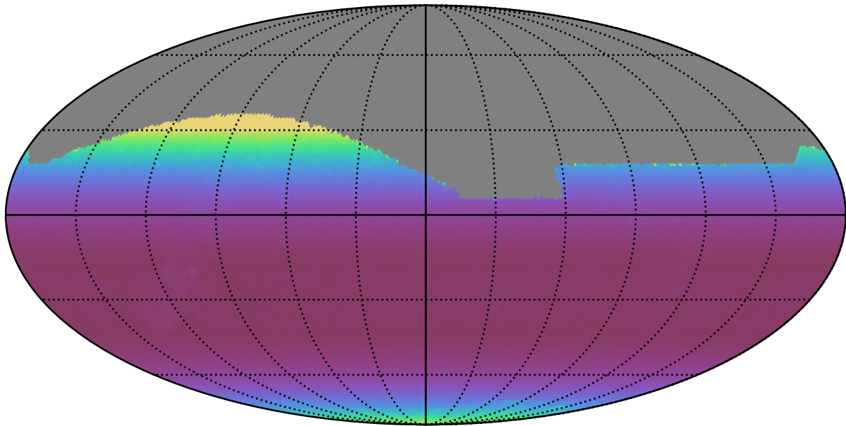
too_elab_r8_d3_ugrizy_v3.4_10yrs All sky z band: Min airmass
